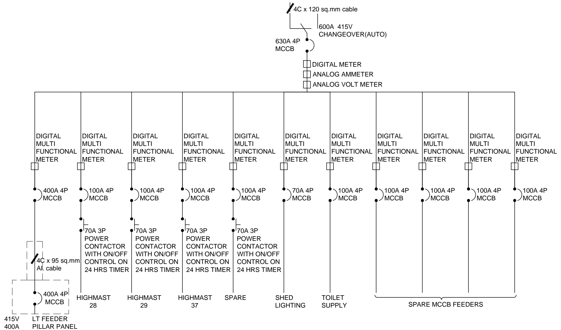
MAIN LT PANEL FOR T3 SHED
