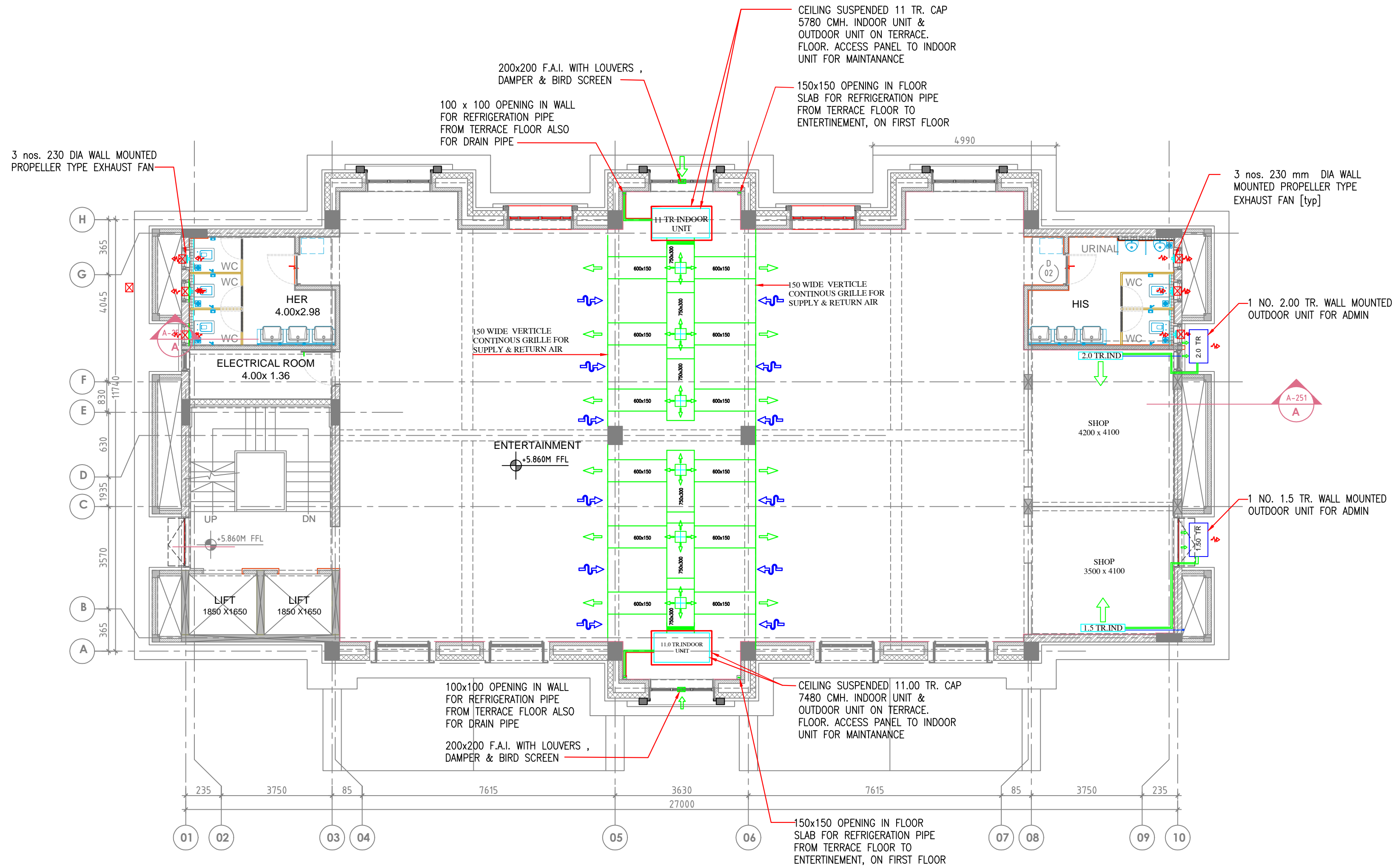
1 FIRST FLOOR PLAN SCALE 1:125
