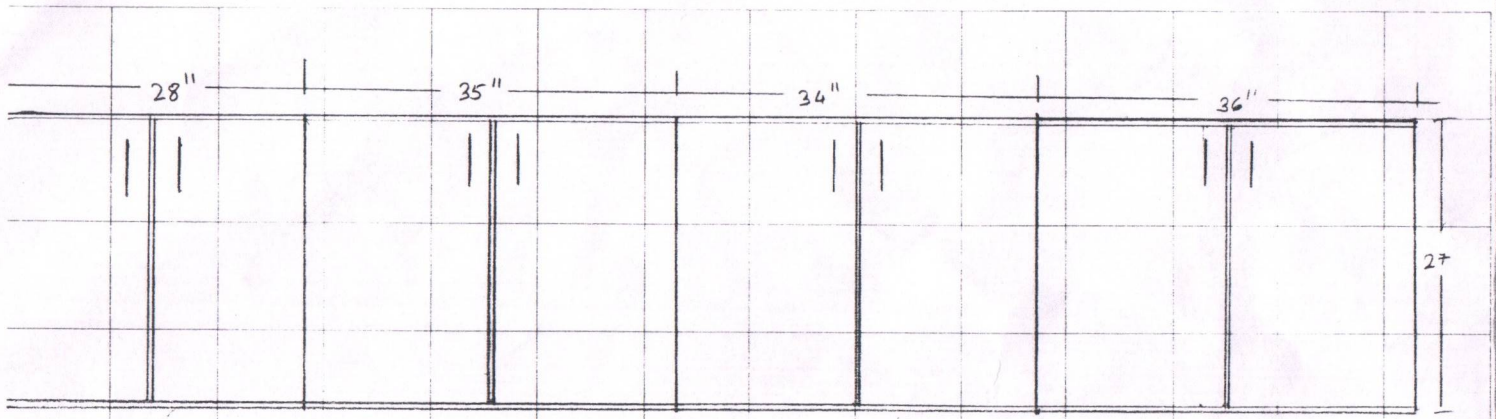
Shutters with frame for existing platform
