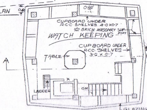
4TH FLOOR PLAN
